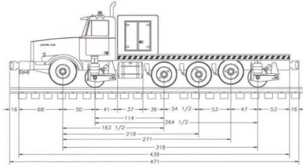
Brandt Power Unit – TANDEM with TAG
