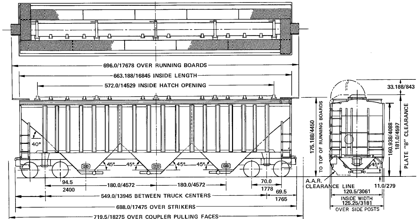
Pullman Standard 4750 cu. ft. Covered Hopper Car.
